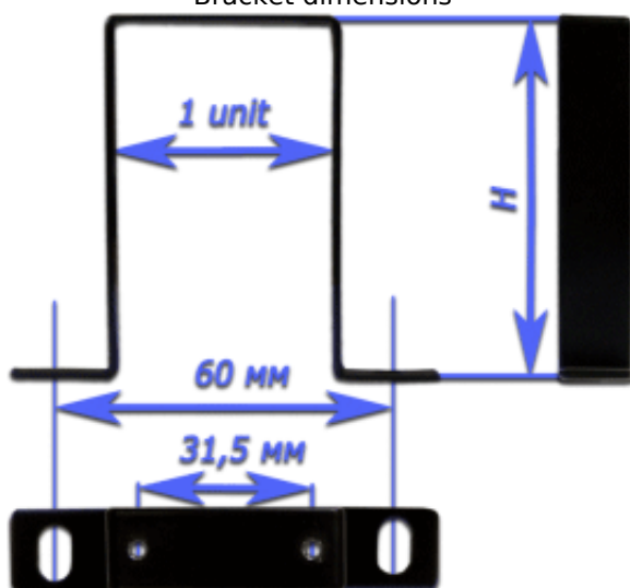
Bracket dimensions
