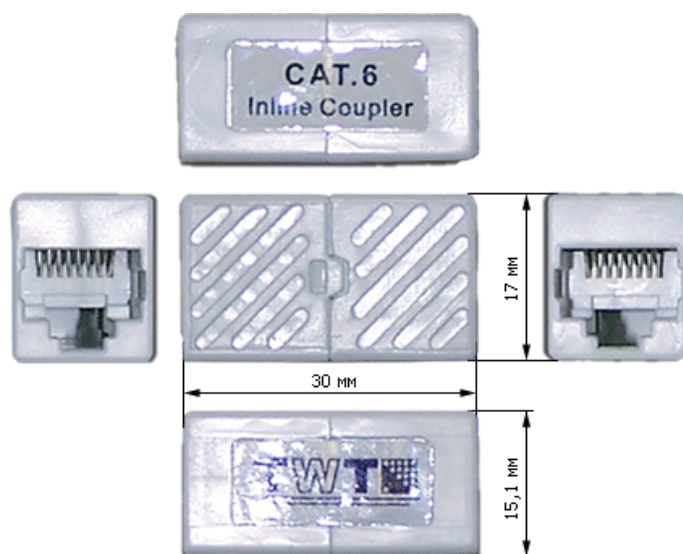
Coupler dimensions
