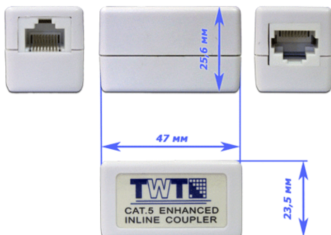
Coupler Dimensions
