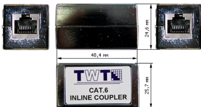
Coupler dimensions
