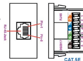
Pinout
