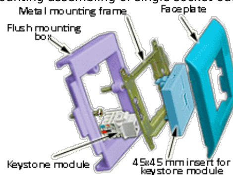
Wall mounting assembling of single socket outlet block
