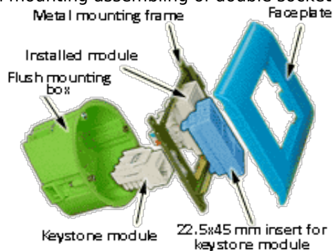
Wall mounting assembling of double socket block
